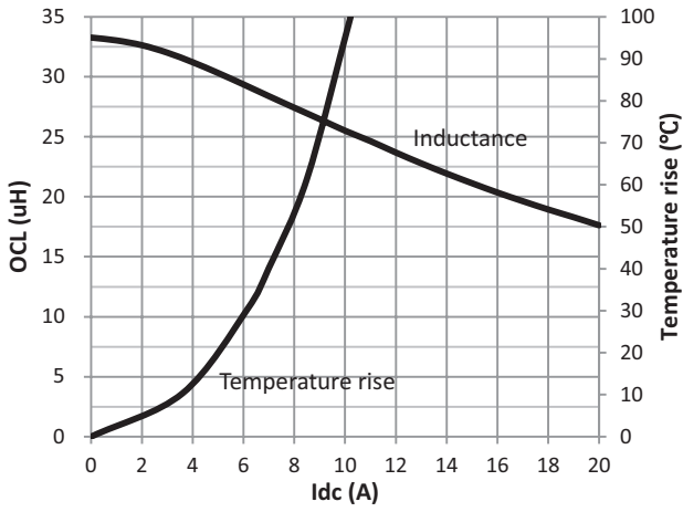
HCM1A1707V2-330-R
