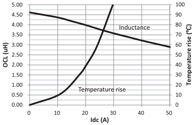
HCM1A1707V2-4R7-R
