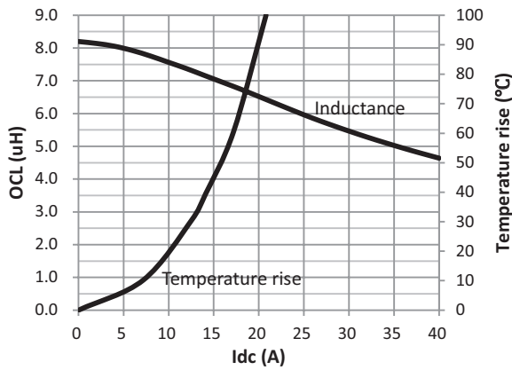
HCM1A1707V2-8R2-R
