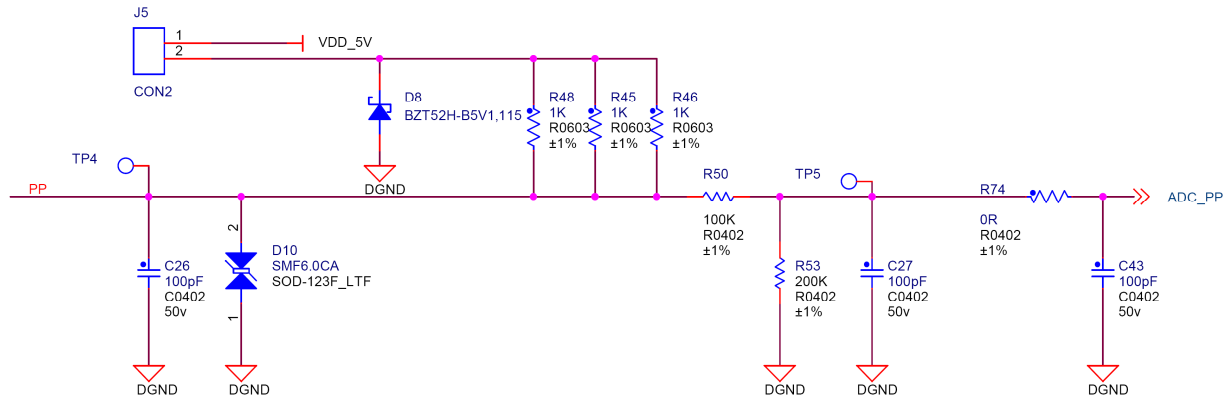
Figure 12 – Proximity Pilot Generation and Measurement
