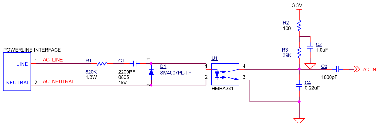
Figure 13 – HPGP Zero Crossing Circuit
