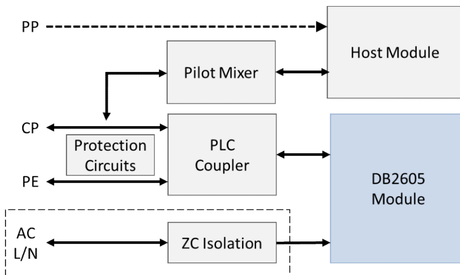
Figure 8 – Control Pilot Signal Managed by Host Module
