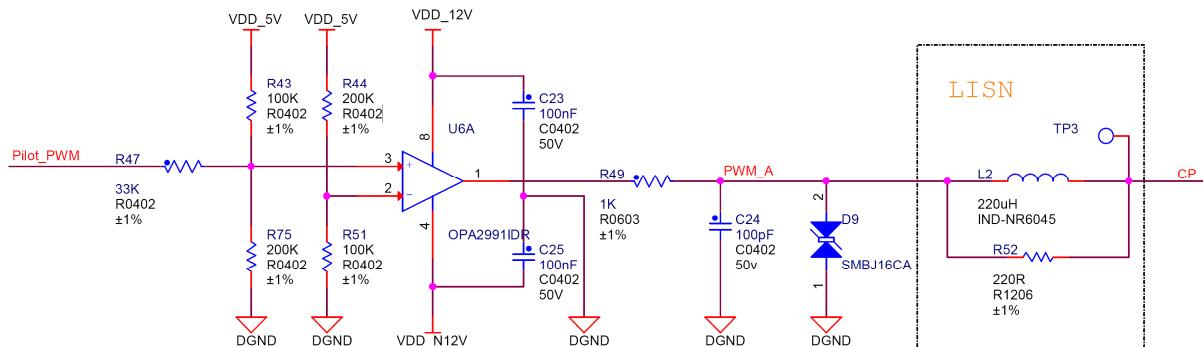
Figure 10 – Control Pilot Signal Generation
