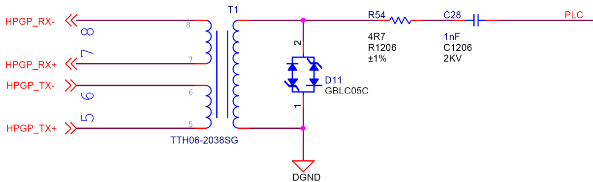
Figure 14 – HPGP Coupler Circuit
