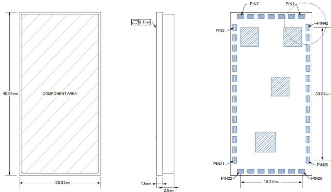
Figure 4 – DB2605 Form Factor
