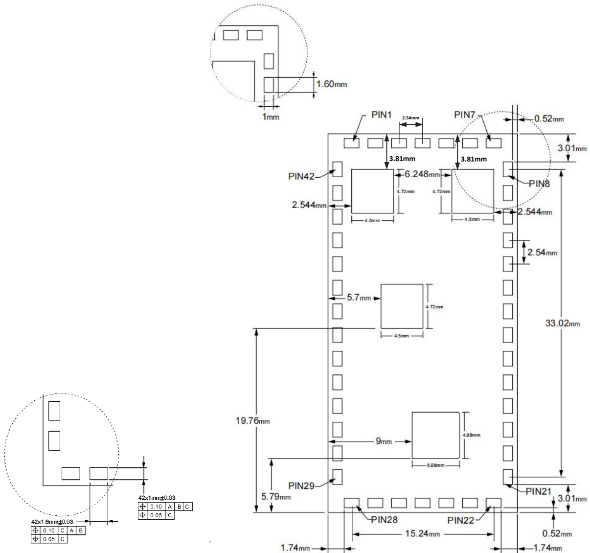
Figure 5 – Recommended Solder Footprint
