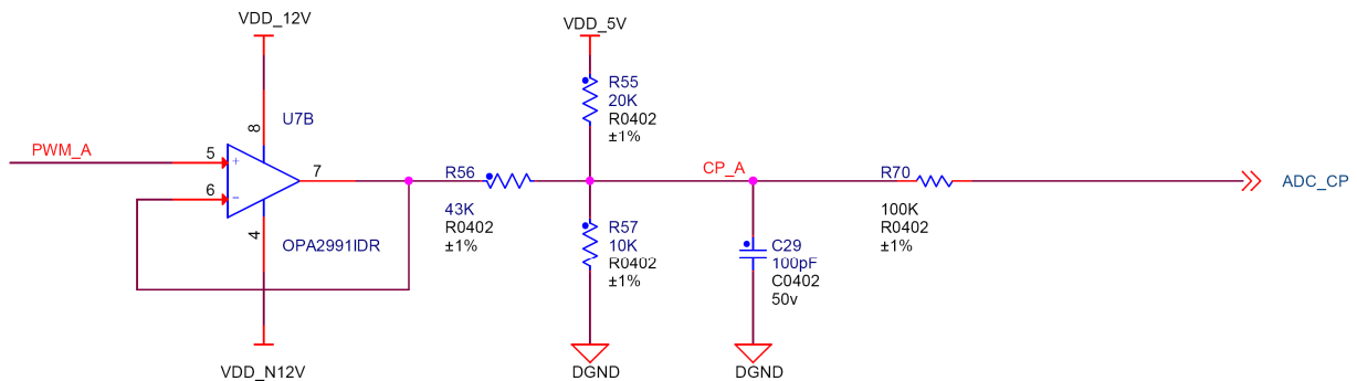
Figure 11 – Control Pilot PWM Voltage Measurement
