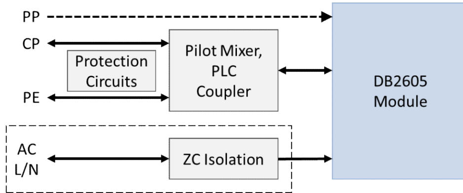
Figure 9 – Control Pilot Signal Managed by DB2605
