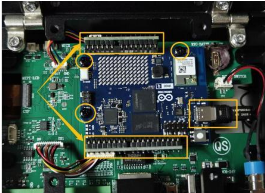
Figure 3-5 Securing the UNO Q and Connecting Cables
