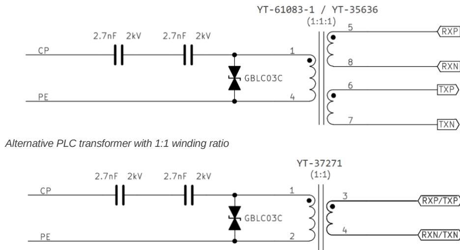
FIGURE 6-1. RED-BEET-E/P 2.0 CIRCUIT FOR COUPLER TO CP/PE
