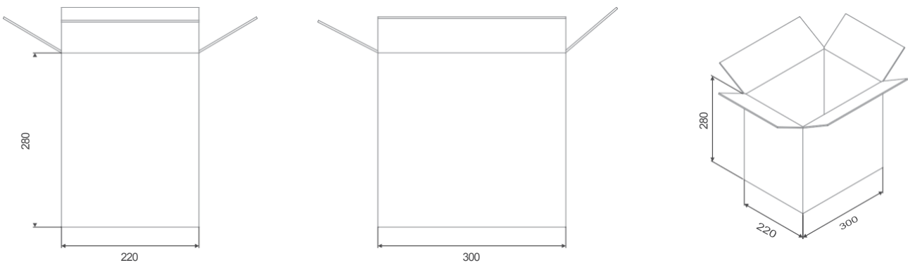
FIGURE 14-2. RED-BEET 2.0 STANDARD PACKING BOX DIMENSIONS
