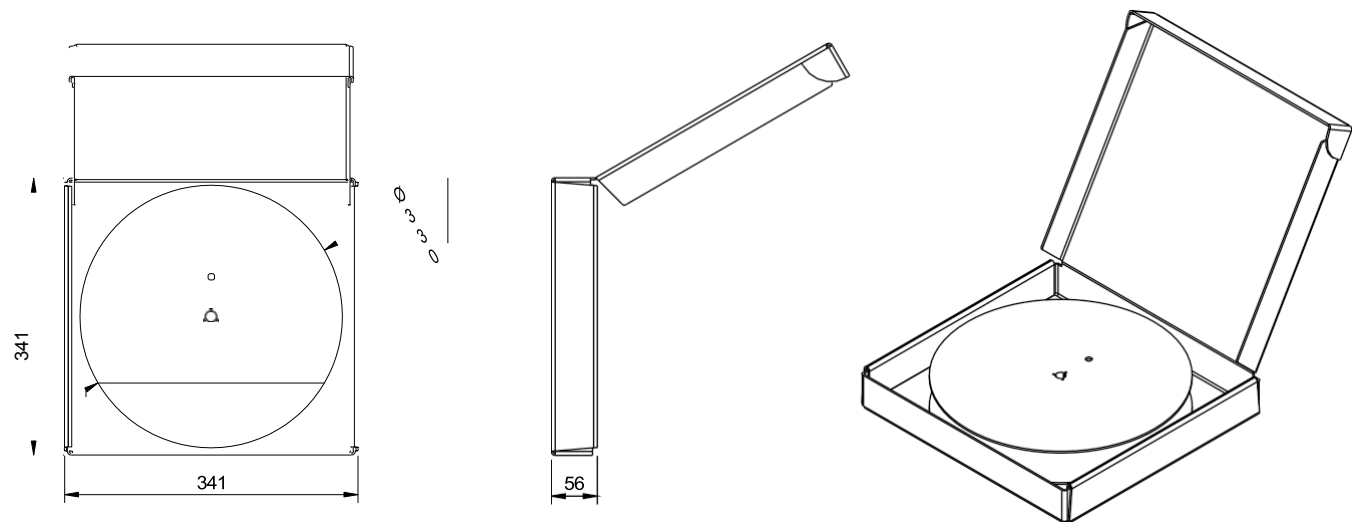
FIGURE 14-5. RED BEET 2.0 REEL PACKAGING BOX WITH REEL
