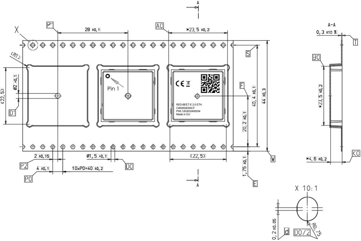
FIGURE 14-3. RED-BEET 2.0 CARRIER TAPE DIMENSIONS
