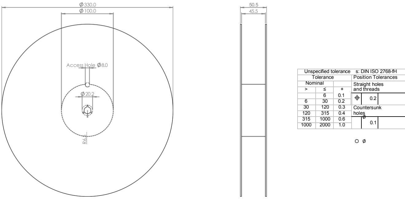
FIGURE 14-4. RED-BEET 2.0 PACKAGING REEL DIMENSIONS
