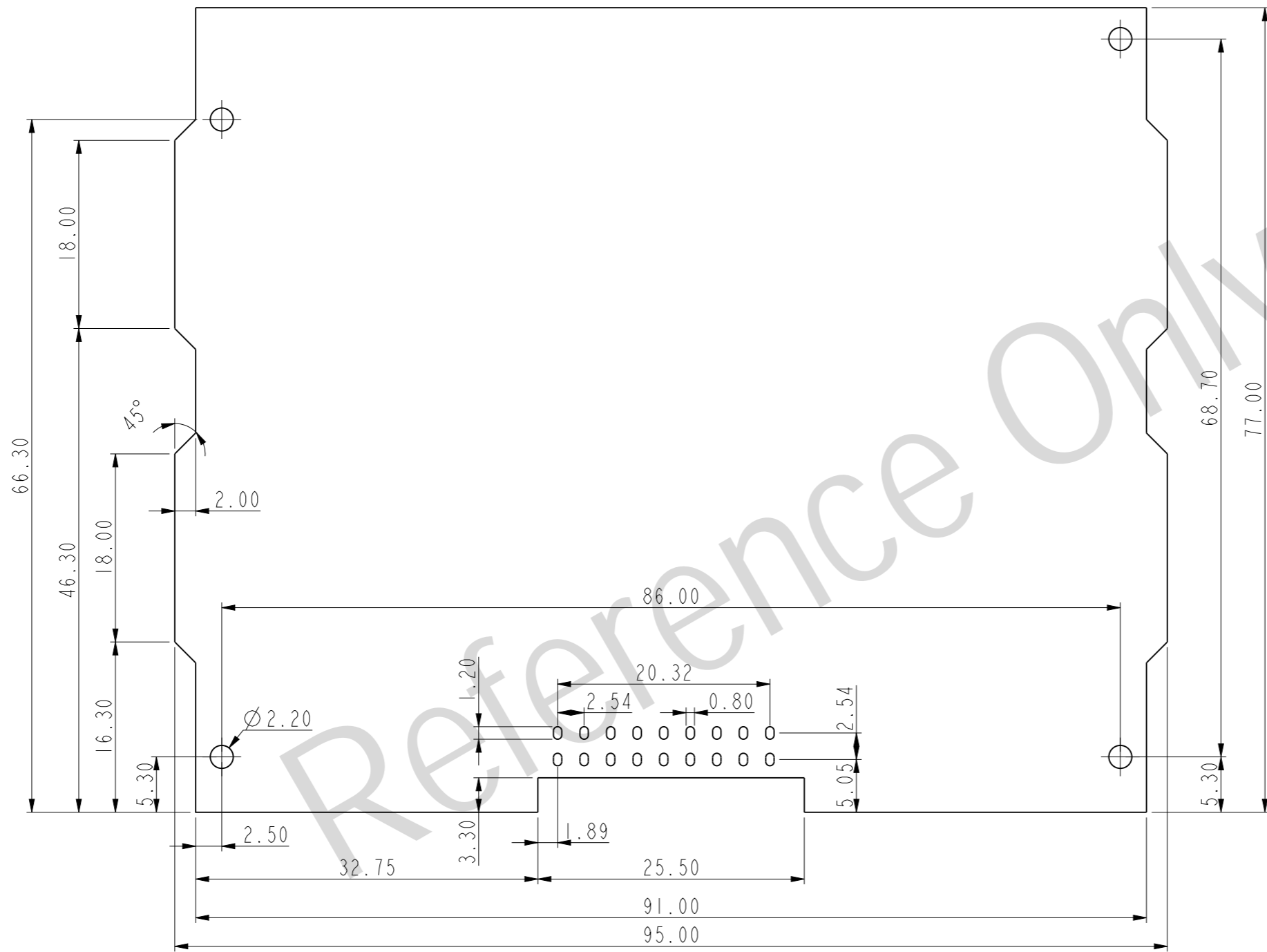
PCB 2 LAYOUT
